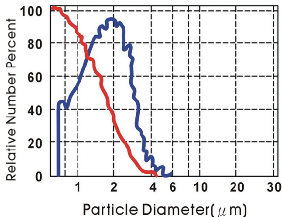
Blue Graph-Particle Size Distribution
